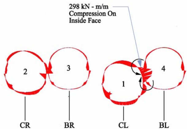
Fig. 5 Calculated Bending Moments in Tunnel Linings for Condition of All Tunnels Excavated, Start of Tunneling, Sta 219+10
