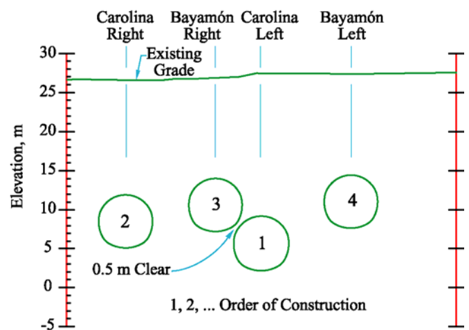
Fig. 4 Tunnel Configuration at Critical Over/Under Condition, Sta 218+70
